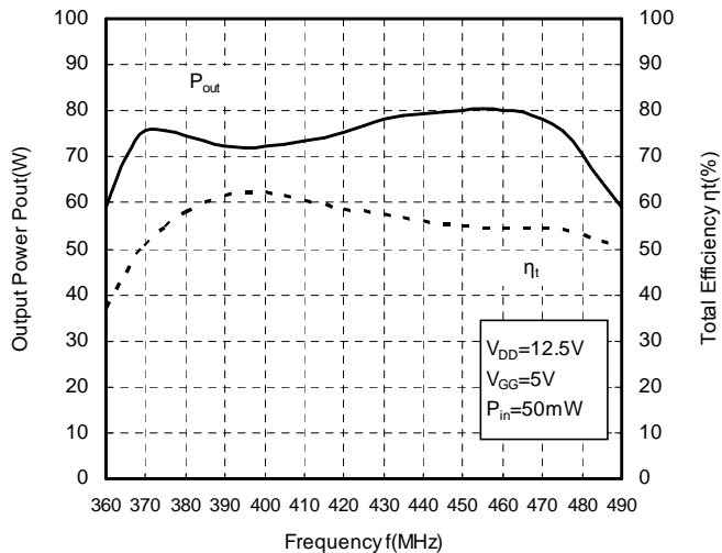
OUTPUT POWER and TOTAL EFFICIENCY, versus FREQUENCY
