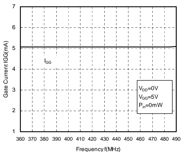
GATE CURRENT versus FREQUENCY
